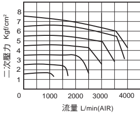
UC-400-02
