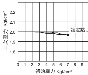
UC-400-03
