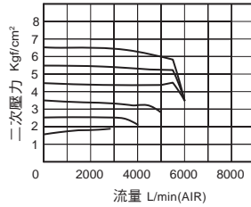
UC-400-03
