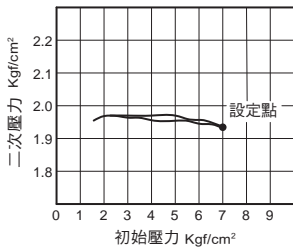
UC-400-02
