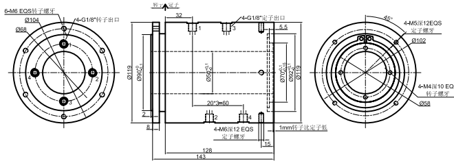
GJ4050-02 尺寸图 4进4出, G1/8接头
